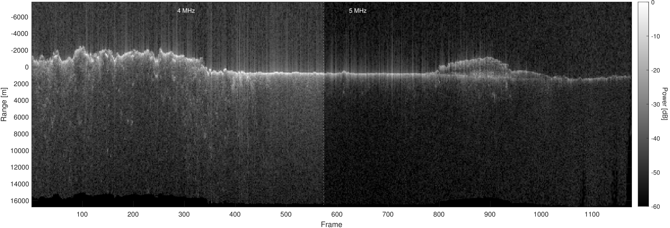
Orbit 5776, Optimized, No Window, Depth-Corrected, Channel 2
