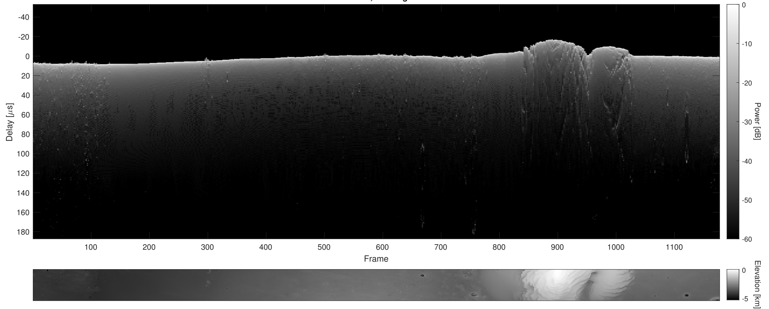
Orbit 5778, Cluttergram
