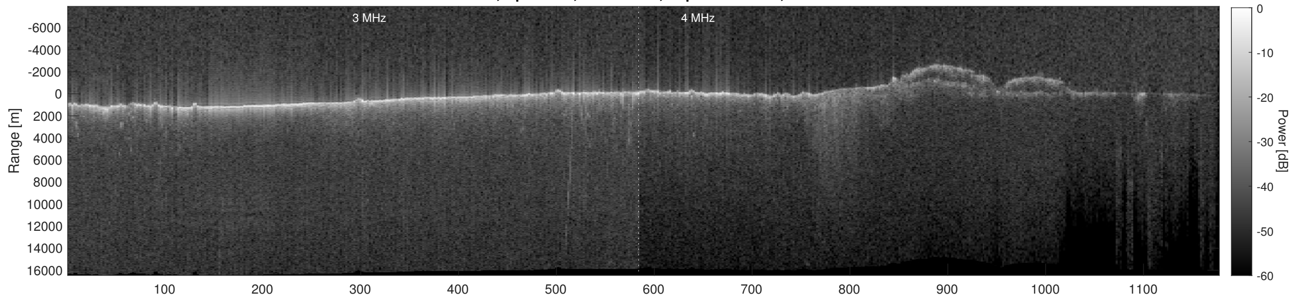
Orbit 5778, Depth-Corrected Cluttergram
