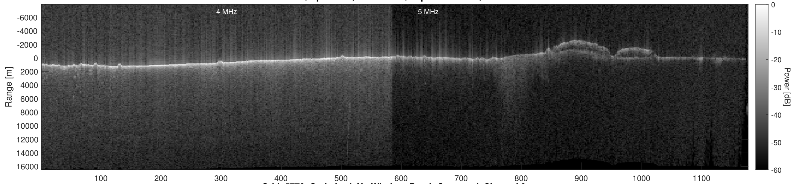
Orbit 5778, Optimized, No Window, Depth-Corrected, Channel 2
