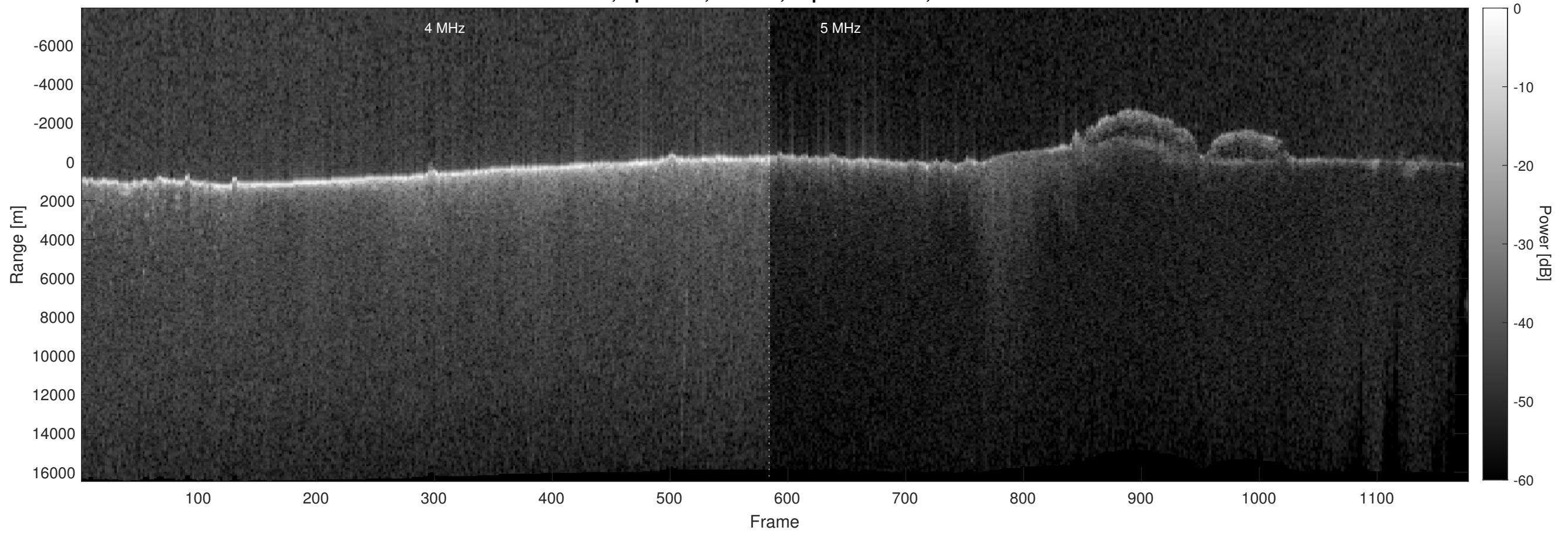
Orbit 5778, Optimized, Window, Depth-Corrected, Channel 2
