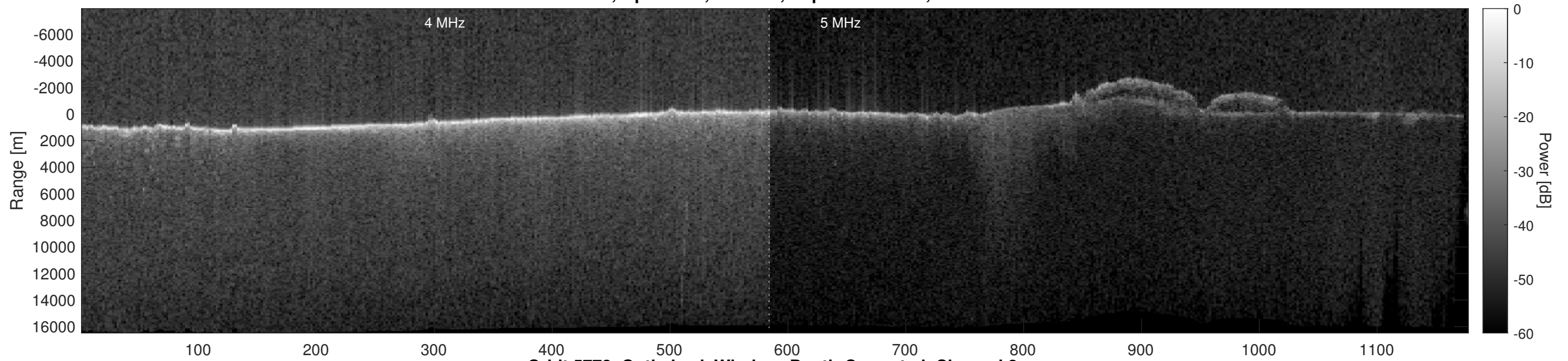
Orbit 5778, Optimized, Window, Depth-Corrected, Channel 2
