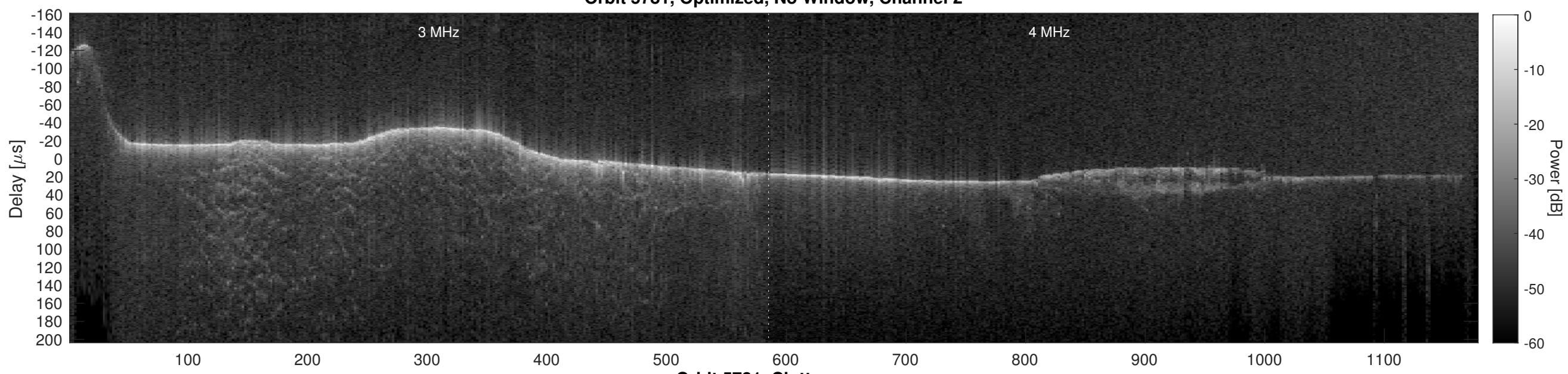
Orbit 5781, Cluttergram
