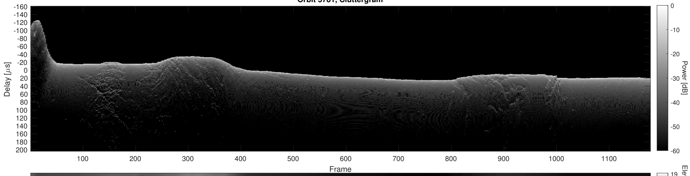
Orbit 5781, Cluttergram
