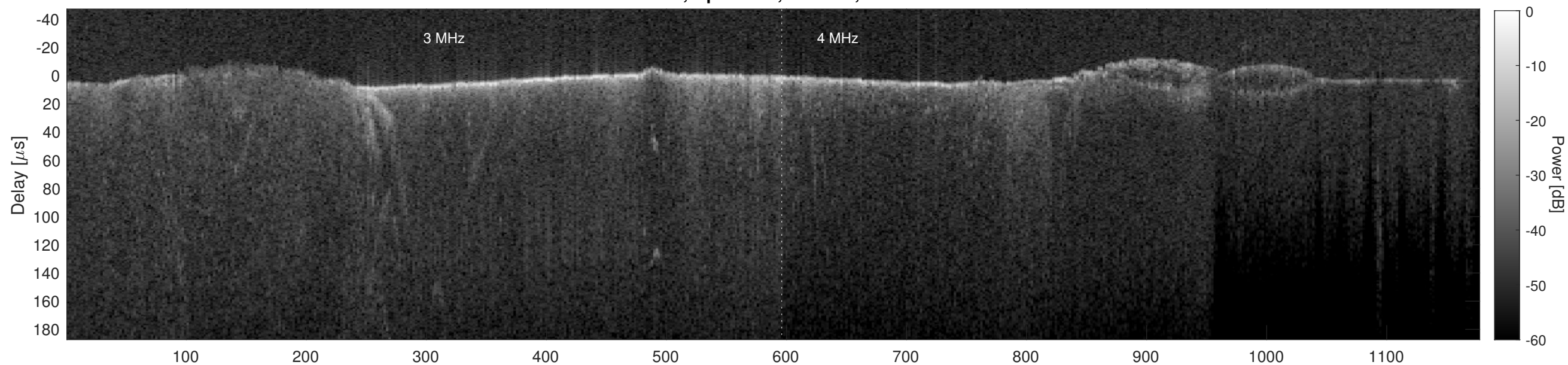
Orbit 5785, Cluttergram
