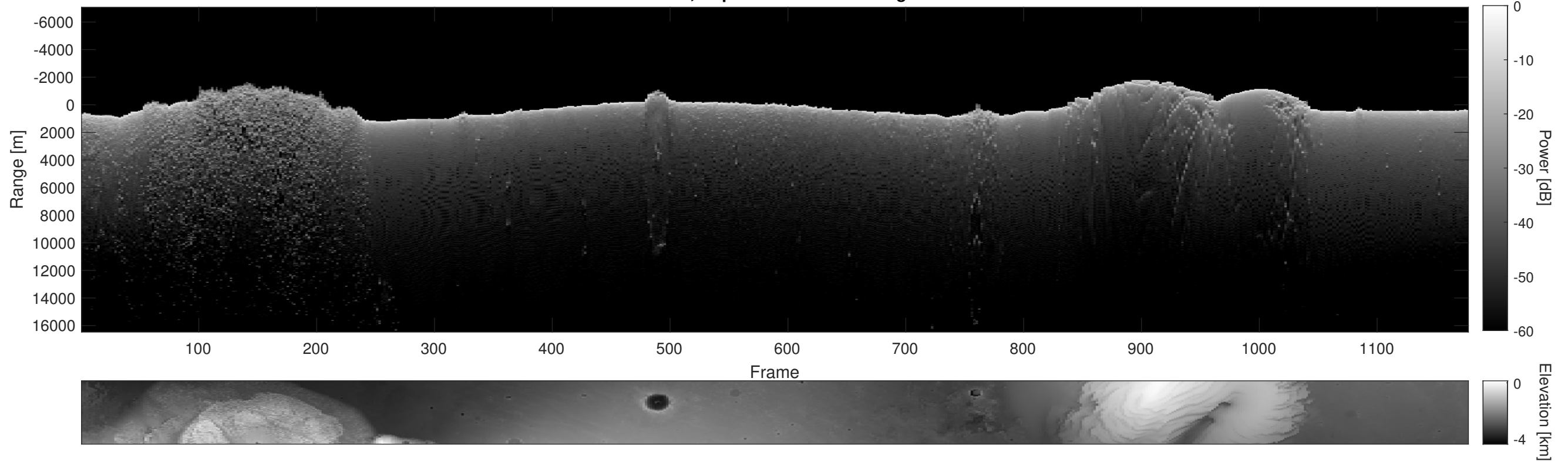
Orbit 5785, Depth-Corrected Cluttergram
