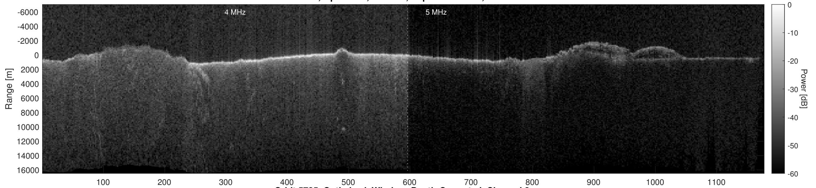
Orbit 5785, Optimized, Window, Depth-Corrected, Channel 2
