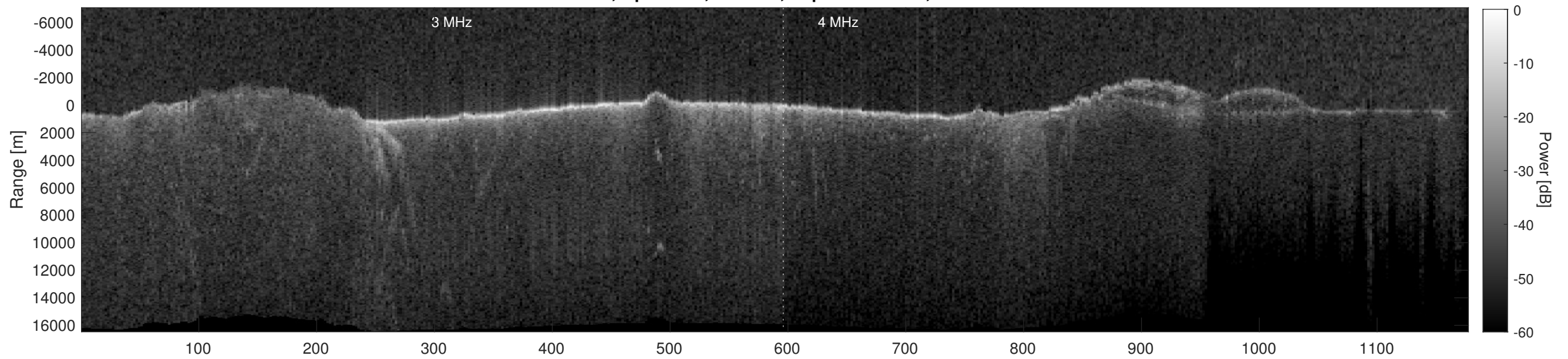
Orbit 5785, Depth-Corrected Cluttergram
