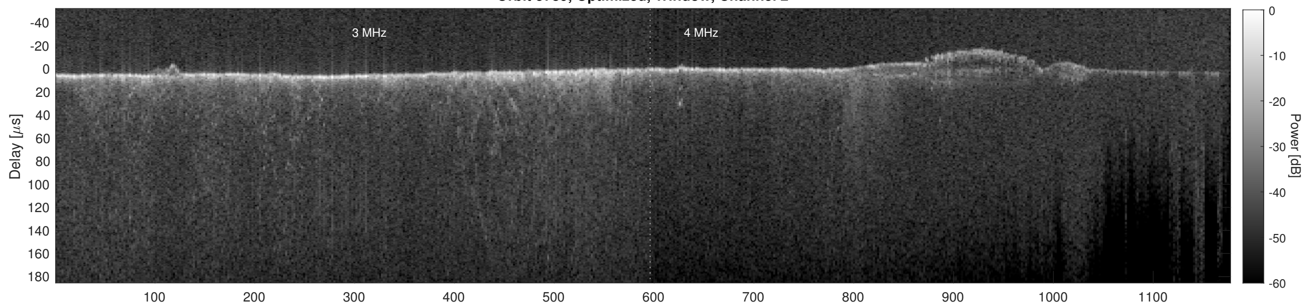
Orbit 5789, Cluttergram
