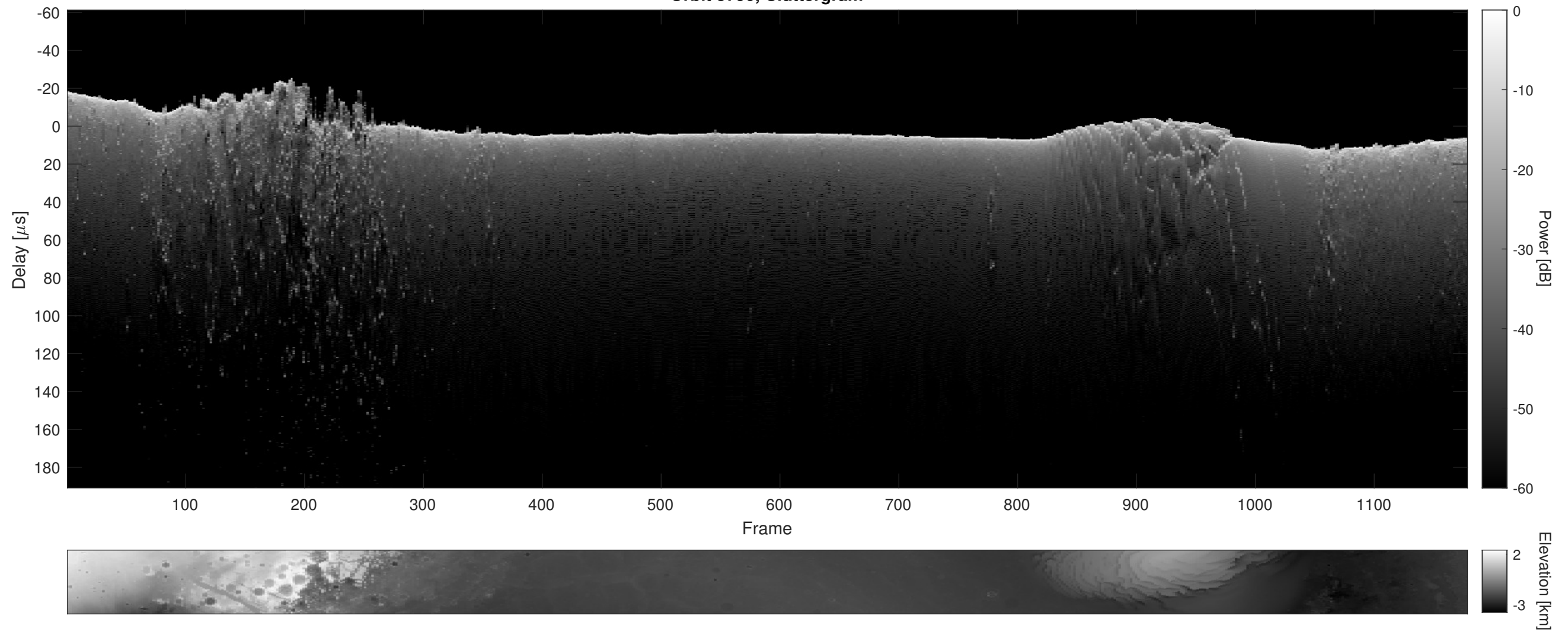
Orbit 5790, Cluttergram
