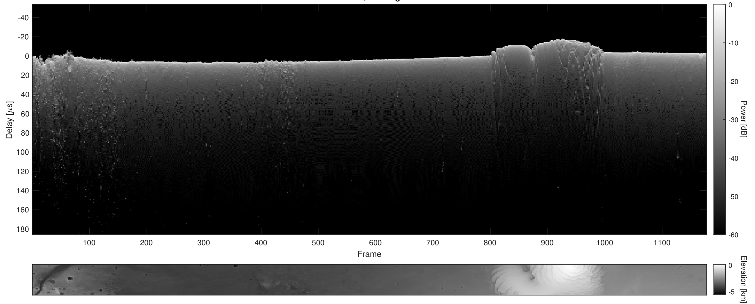
Orbit 5791, Cluttergram
