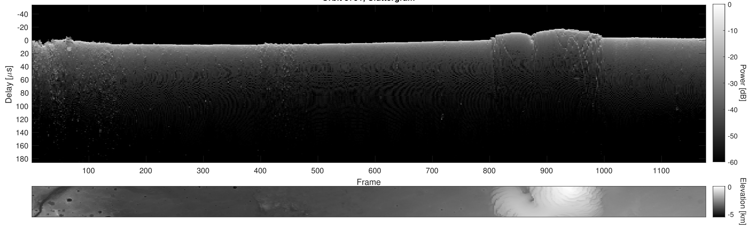
Orbit 5791, Cluttergram
