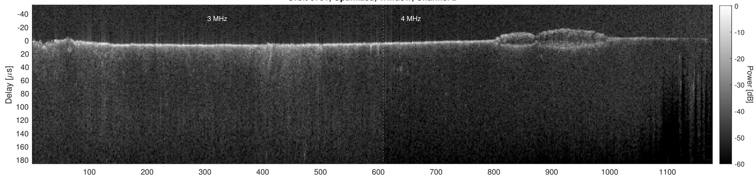
Orbit 5791, Cluttergram
