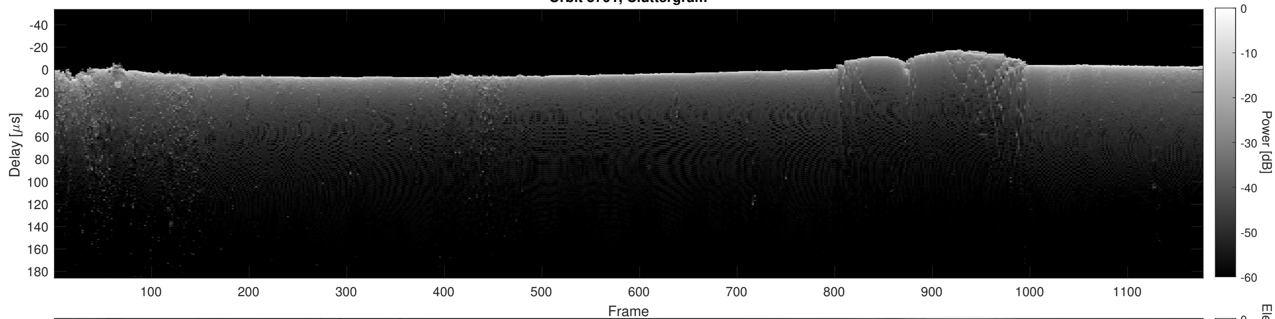
Orbit 5791, Cluttergram
