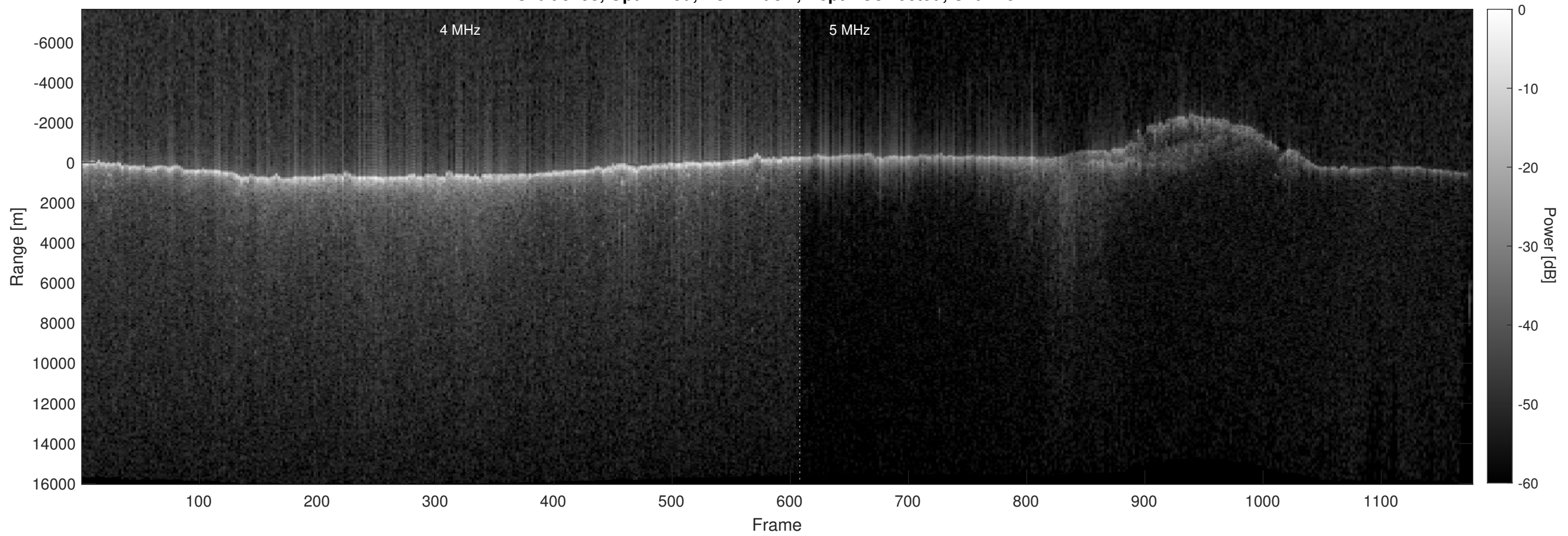
Orbit 5793, Optimized, No Window, Depth-Corrected, Channel 2
