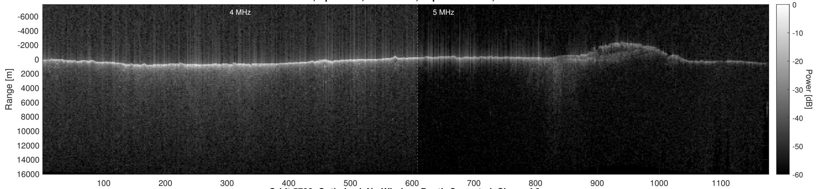
Orbit 5793, Optimized, No Window, Depth-Corrected, Channel 2
