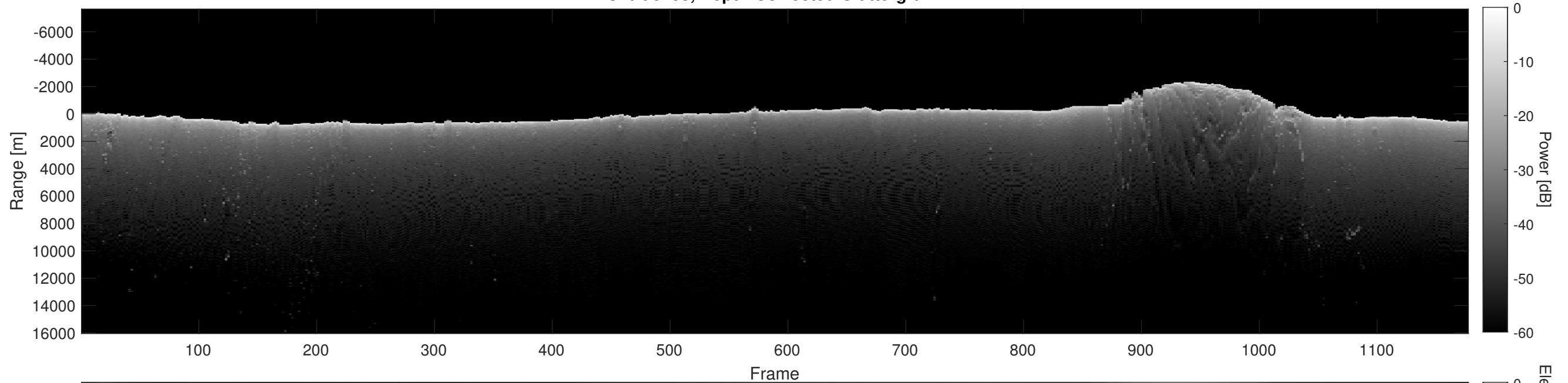
Orbit 5793, Depth-Corrected Cluttergram
