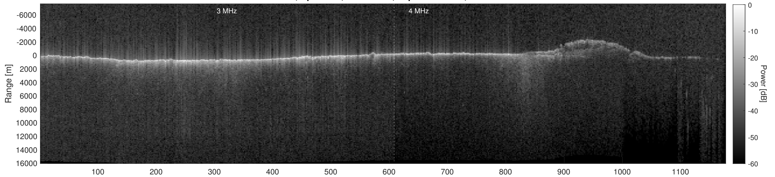
Orbit 5793, Depth-Corrected Cluttergram
