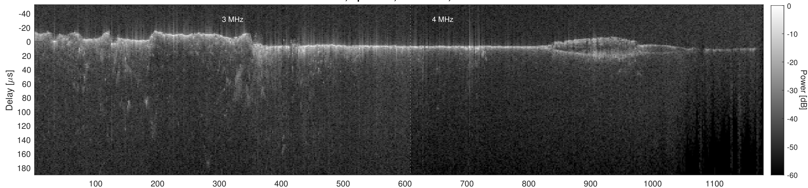
Orbit 5794, Cluttergram
