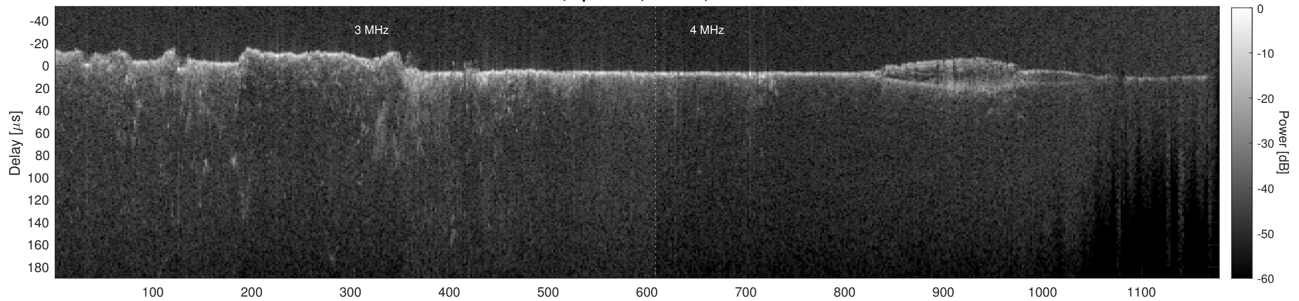
Orbit 5794, Cluttergram
