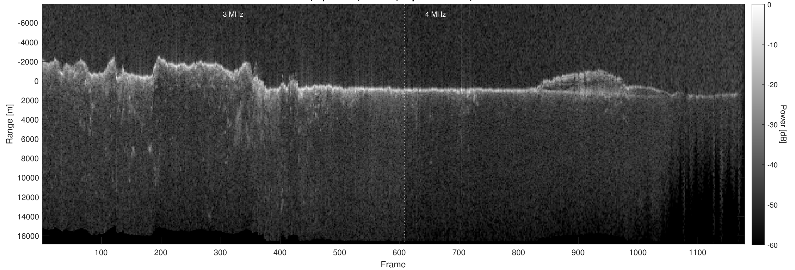
Orbit 5794, Optimized, Window, Depth-Corrected, Channel 2
