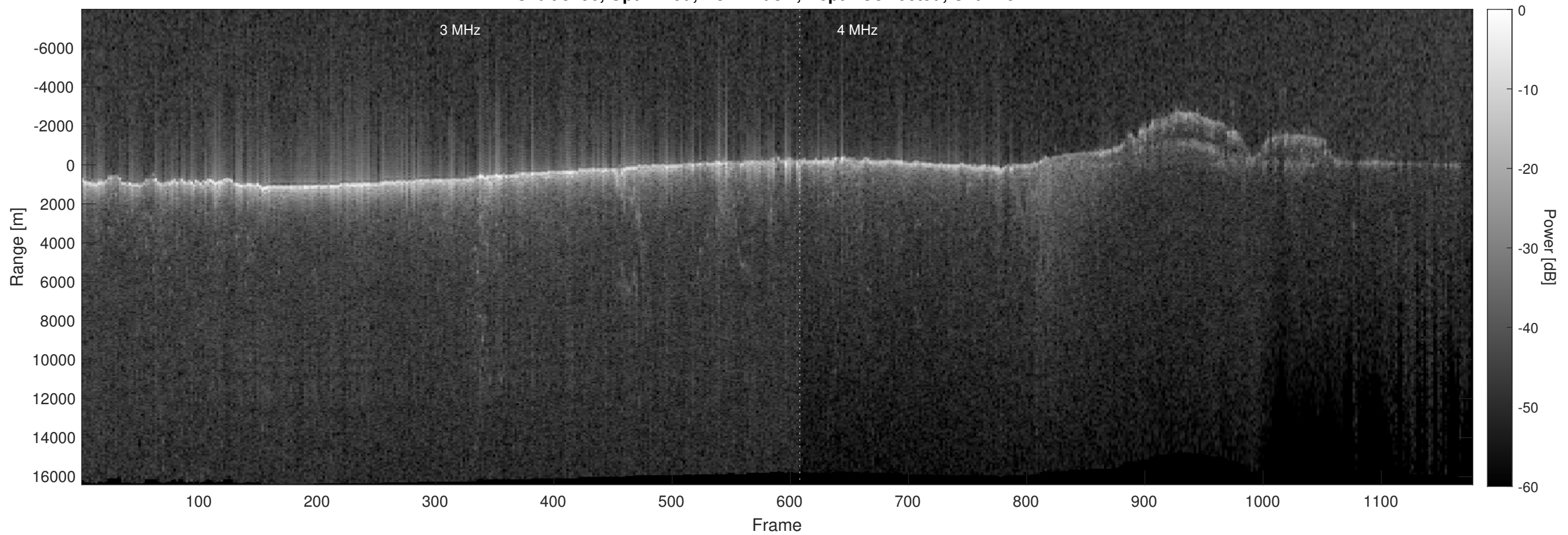
Orbit 5796, Optimized, No Window, Depth-Corrected, Channel 2
