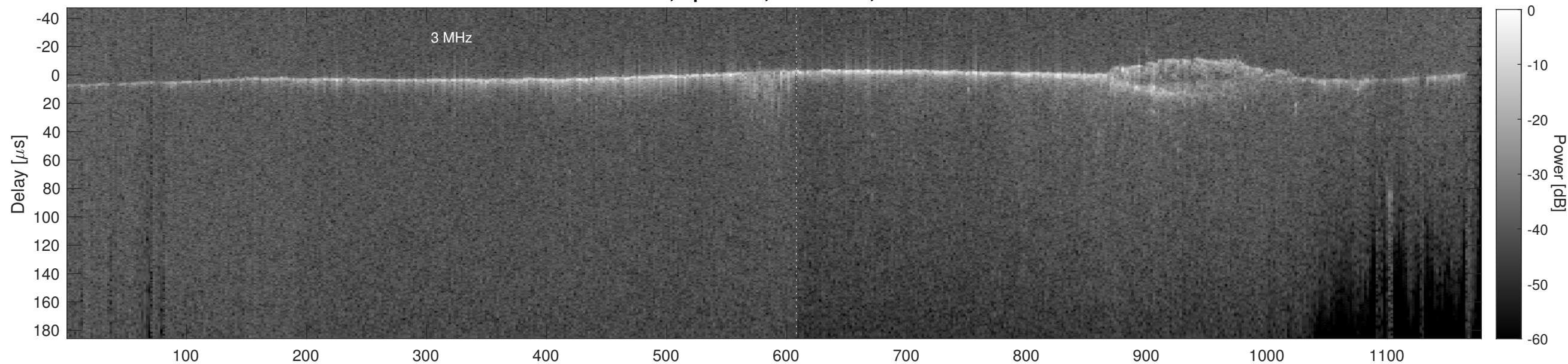
Orbit 5797, Cluttergram
