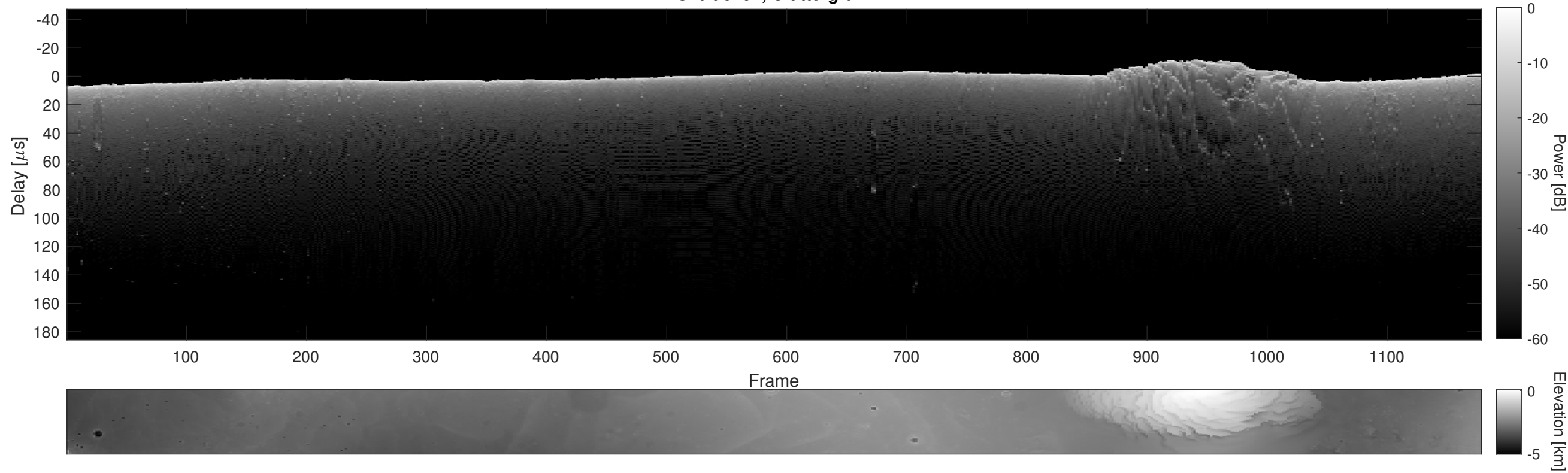
Orbit 5797, Cluttergram
