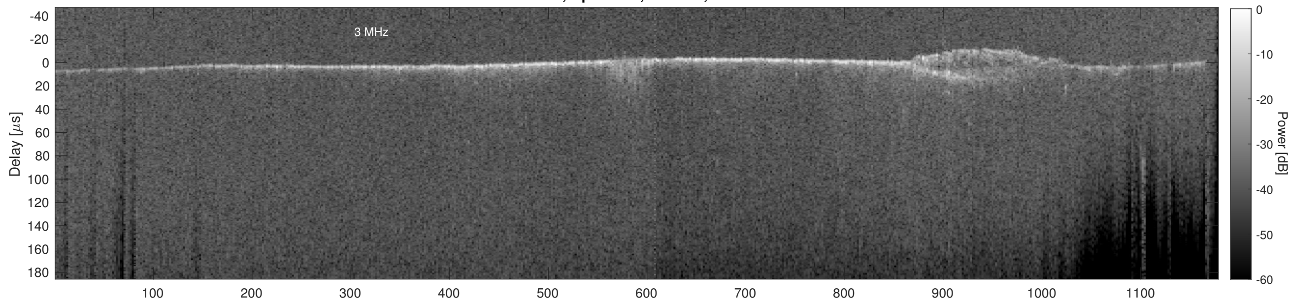
Orbit 5797, Cluttergram
