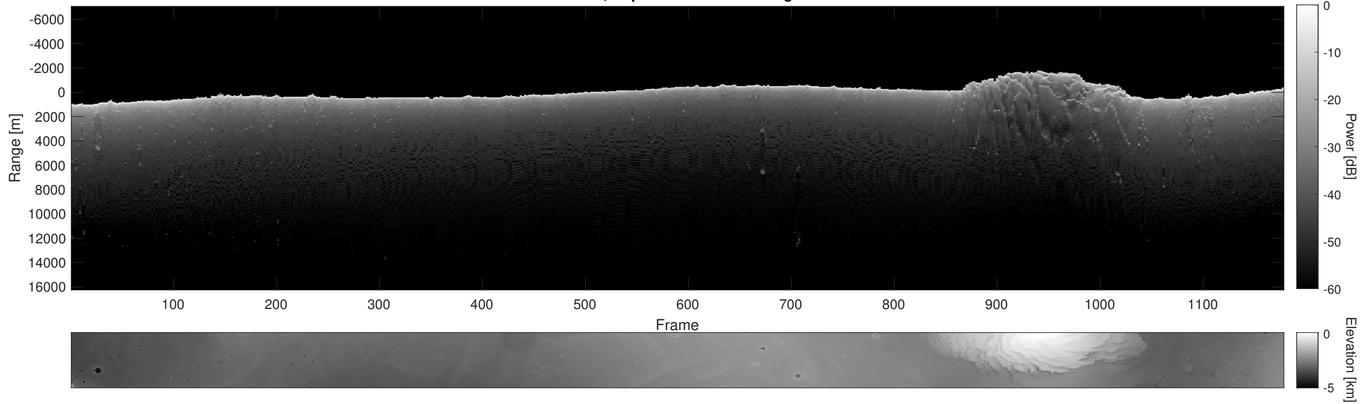
Orbit 5797, Depth-Corrected Cluttergram
