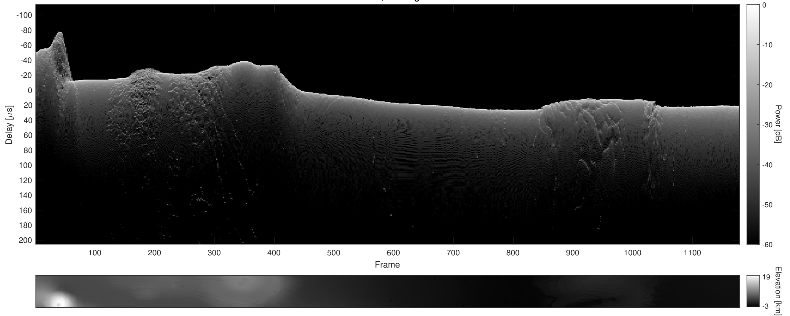
Orbit 5799, Cluttergram
