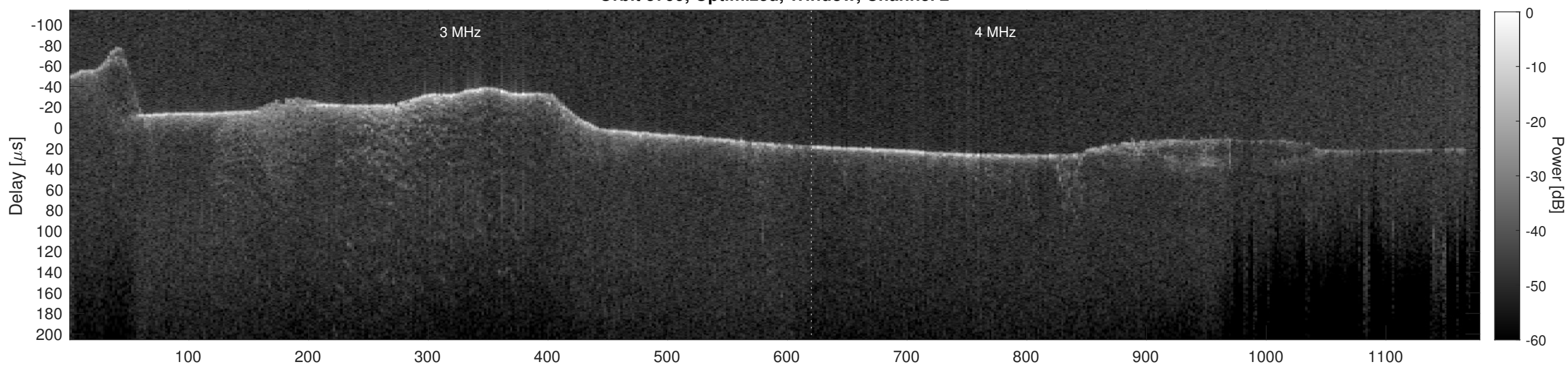
Orbit 5799, Cluttergram
