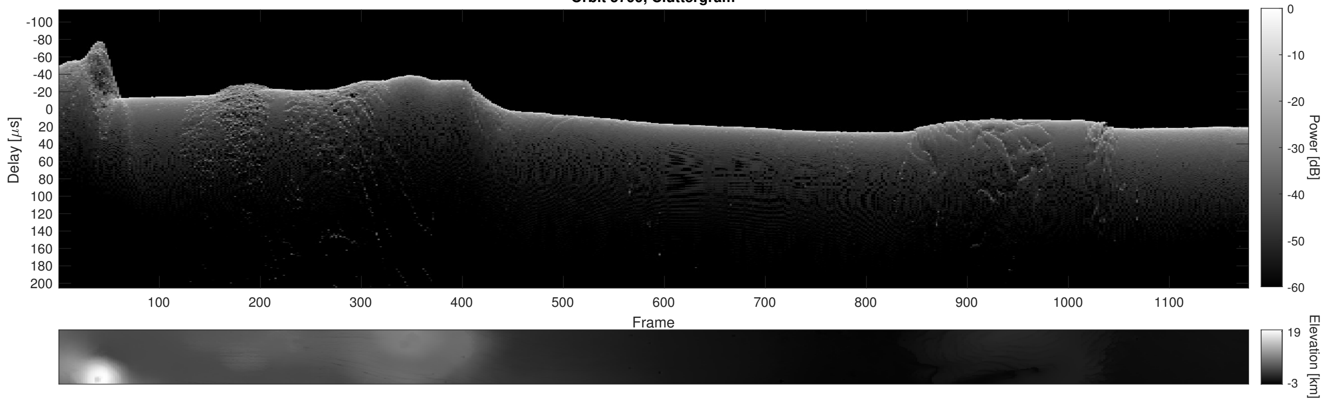
Orbit 5799, Cluttergram
