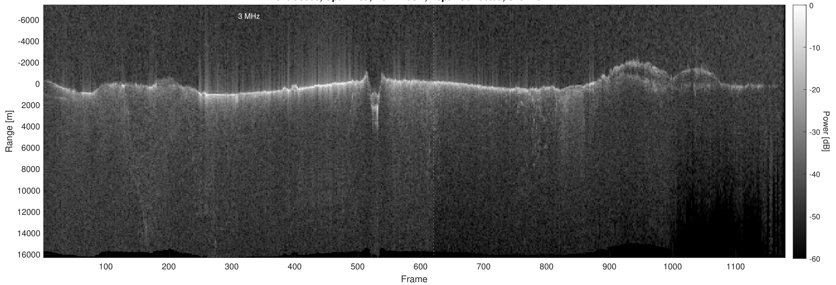
Orbit 5803, Optimized, No Window, Depth-Corrected, Channel 2
