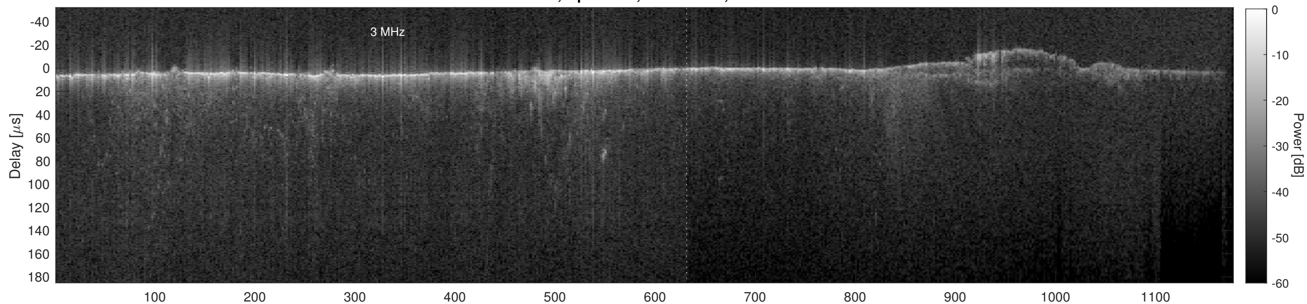
Orbit 5807, Cluttergram
