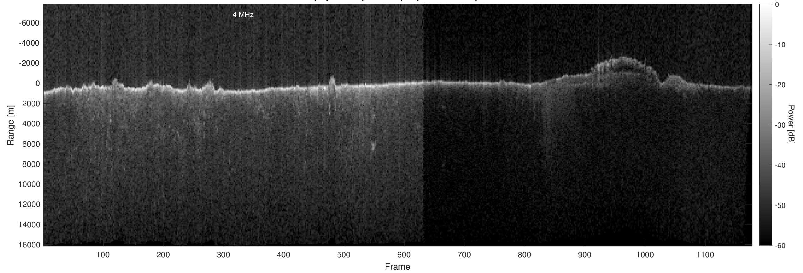
Orbit 5807, Optimized, Window, Depth-Corrected, Channel 2
