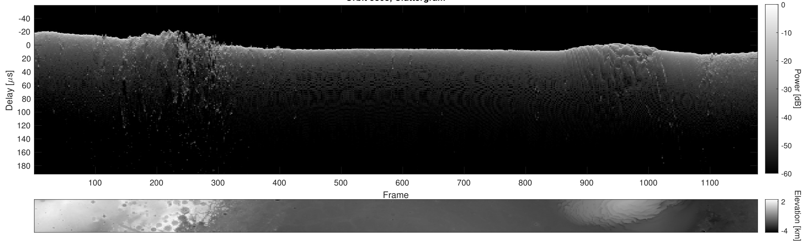
Orbit 5808, Cluttergram
