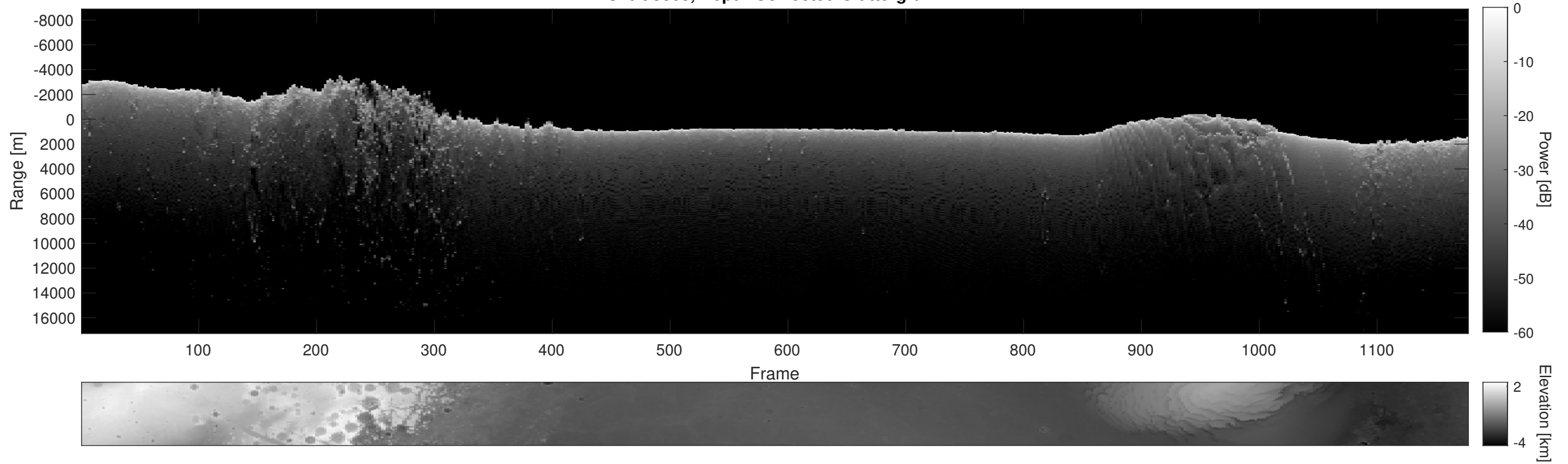
Orbit 5808, Depth-Corrected Cluttergram
