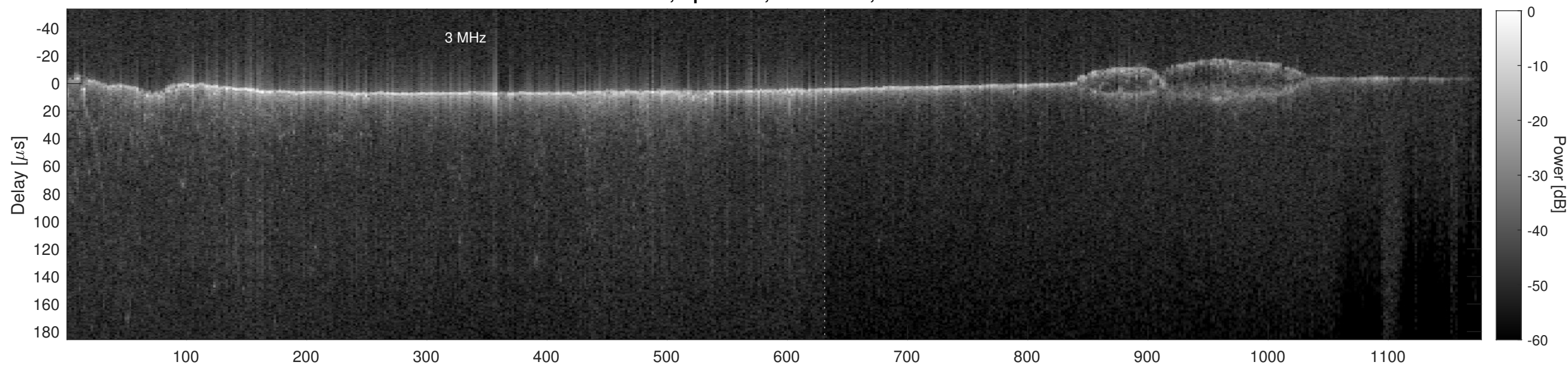
Orbit 5809, Cluttergram
