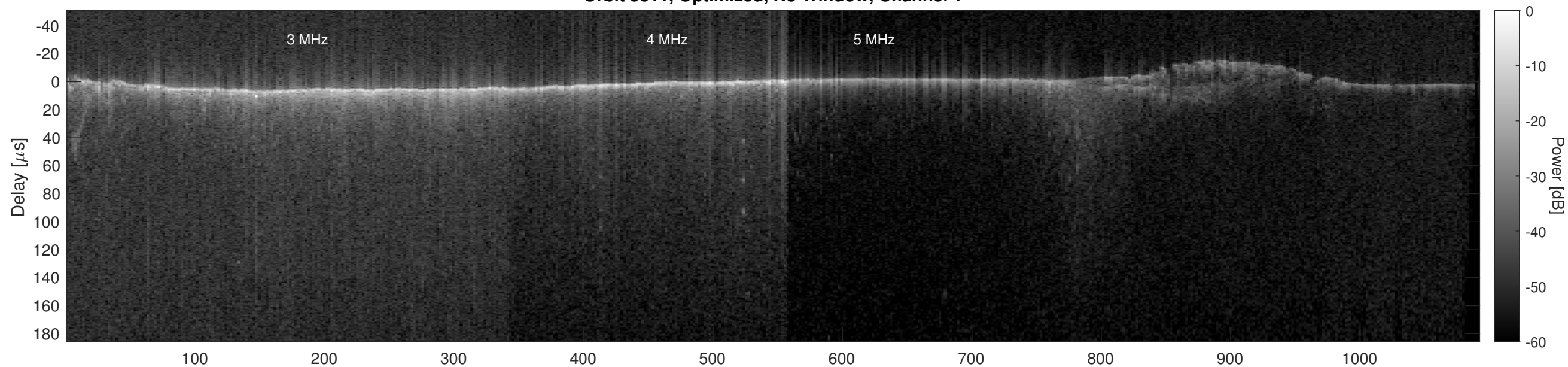
Orbit 5811, Optimized, No Window, Channel 2
