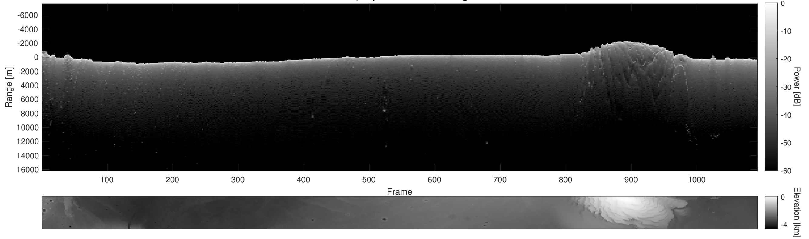
Orbit 5811, Depth-Corrected Cluttergram
