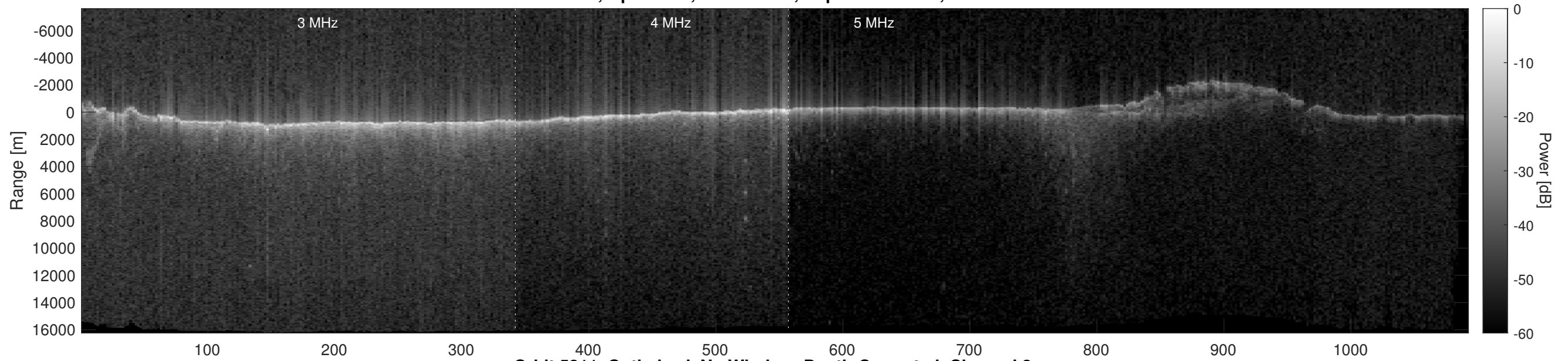
Orbit 5811, Optimized, No Window, Depth-Corrected, Channel 2
