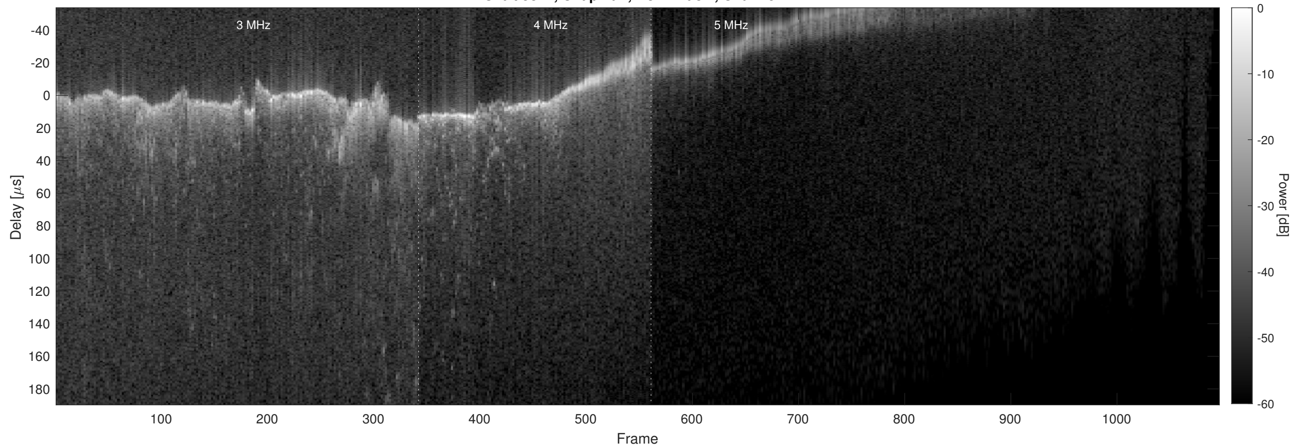
Orbit 5812, Chapman, No Window, Channel 2
