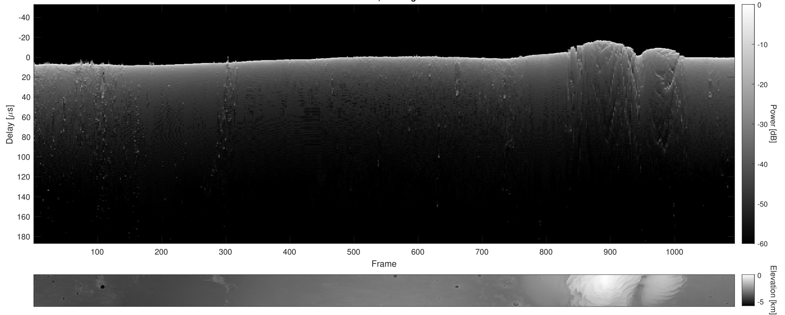
Orbit 5814, Cluttergram
