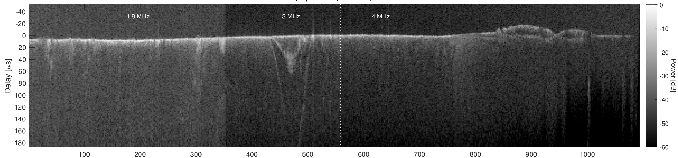
Orbit 5814, Cluttergram
