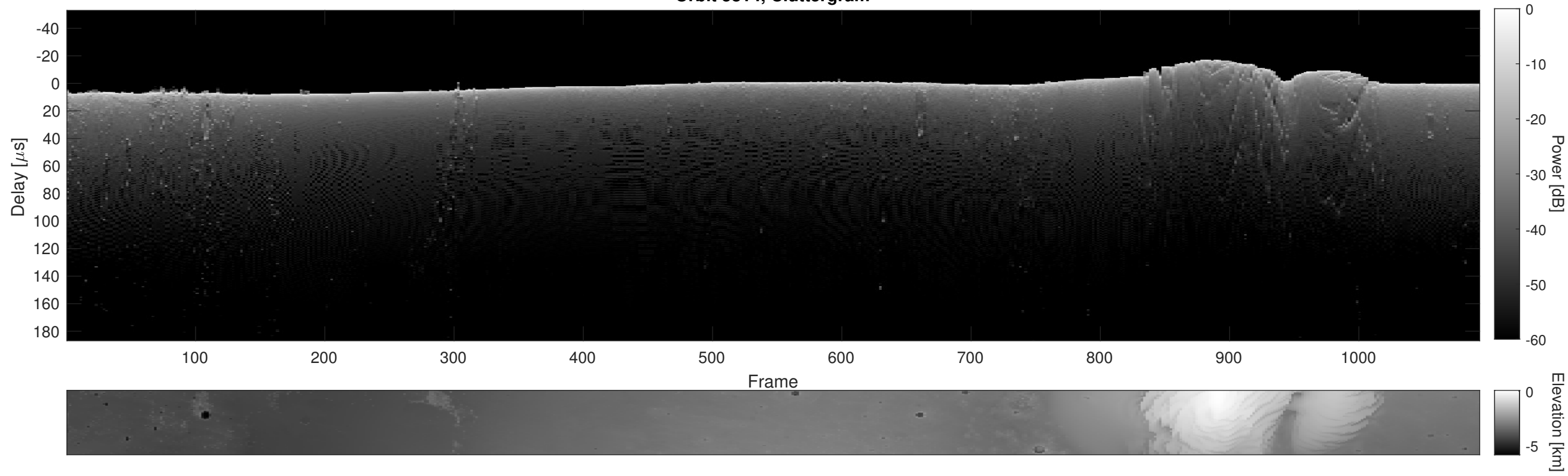
Orbit 5814, Cluttergram
