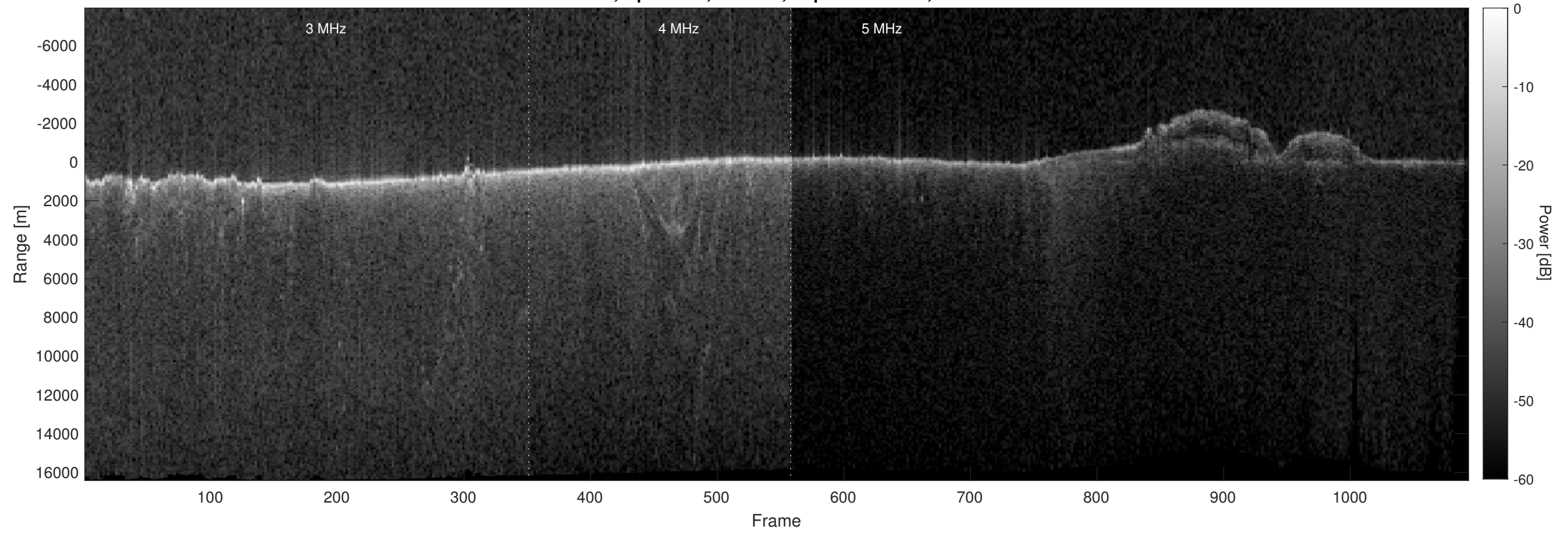
Orbit 5814, Optimized, Window, Depth-Corrected, Channel 2
