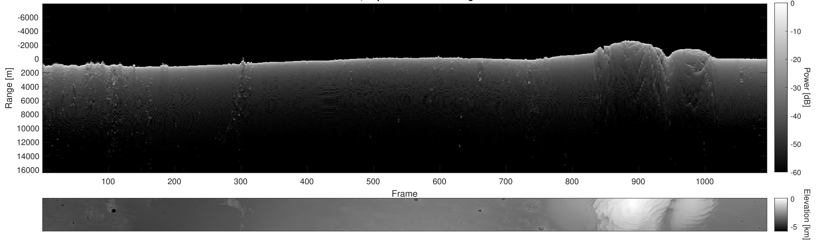
Orbit 5814, Depth-Corrected Cluttergram
