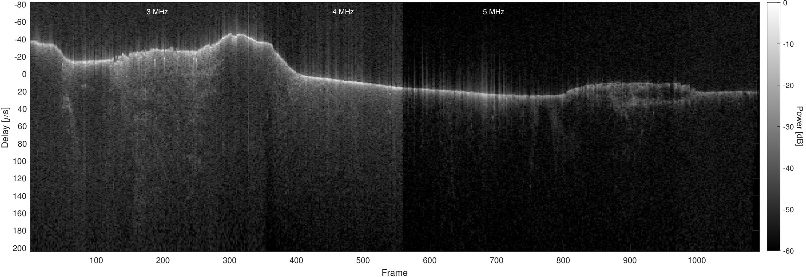
Orbit 5817, Optimized, No Window, Channel 2
