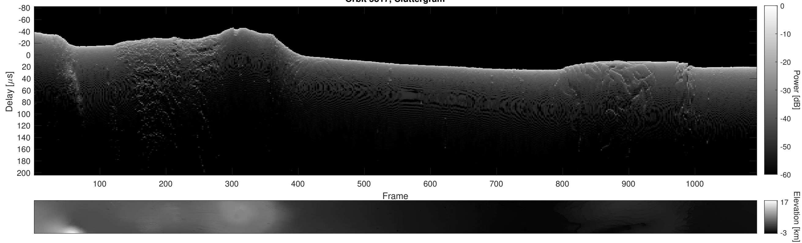
Orbit 5817, Cluttergram
