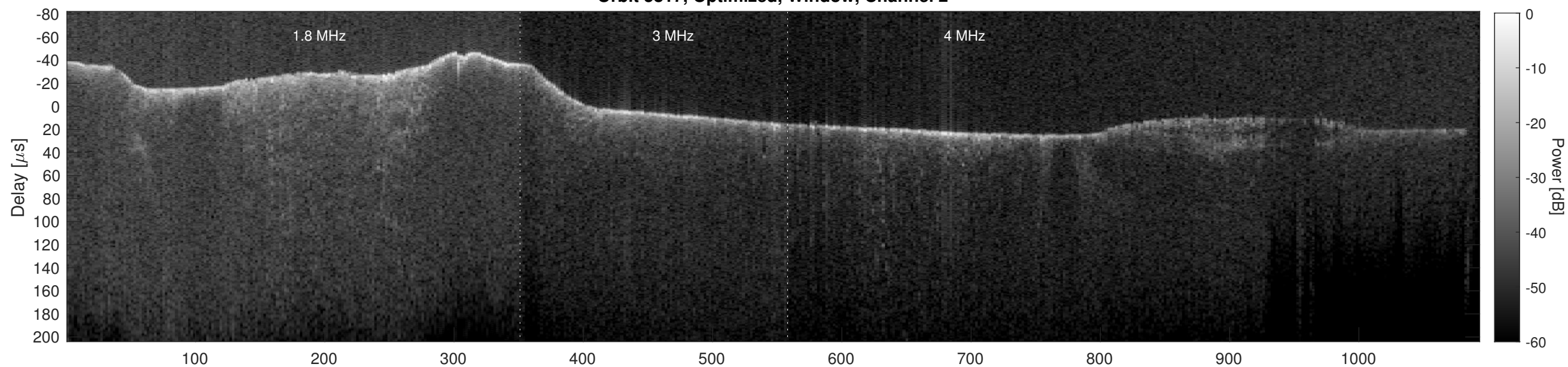
Orbit 5817, Cluttergram
