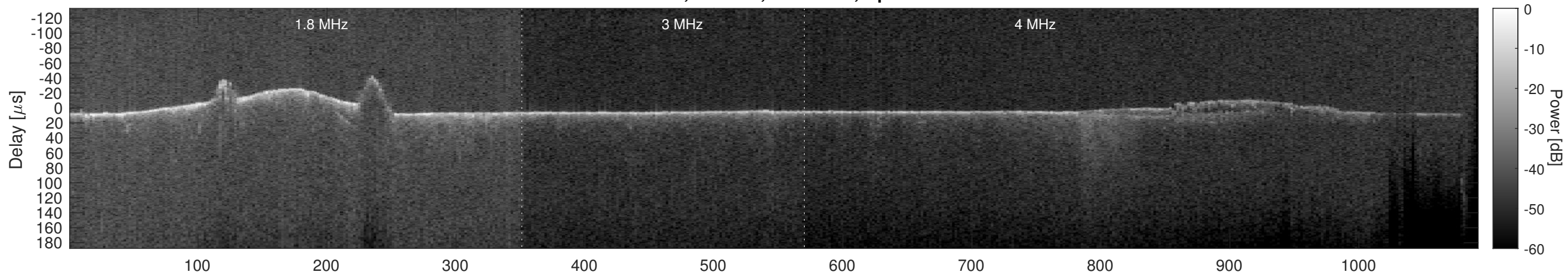
Orbit 5818, Cluttergram
