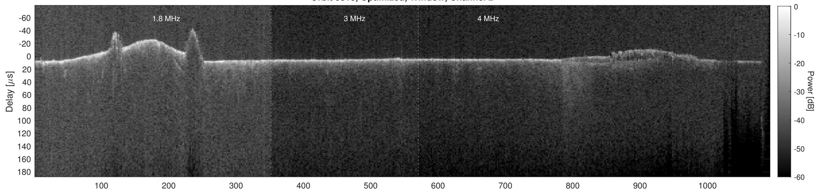
Orbit 5818, Cluttergram
