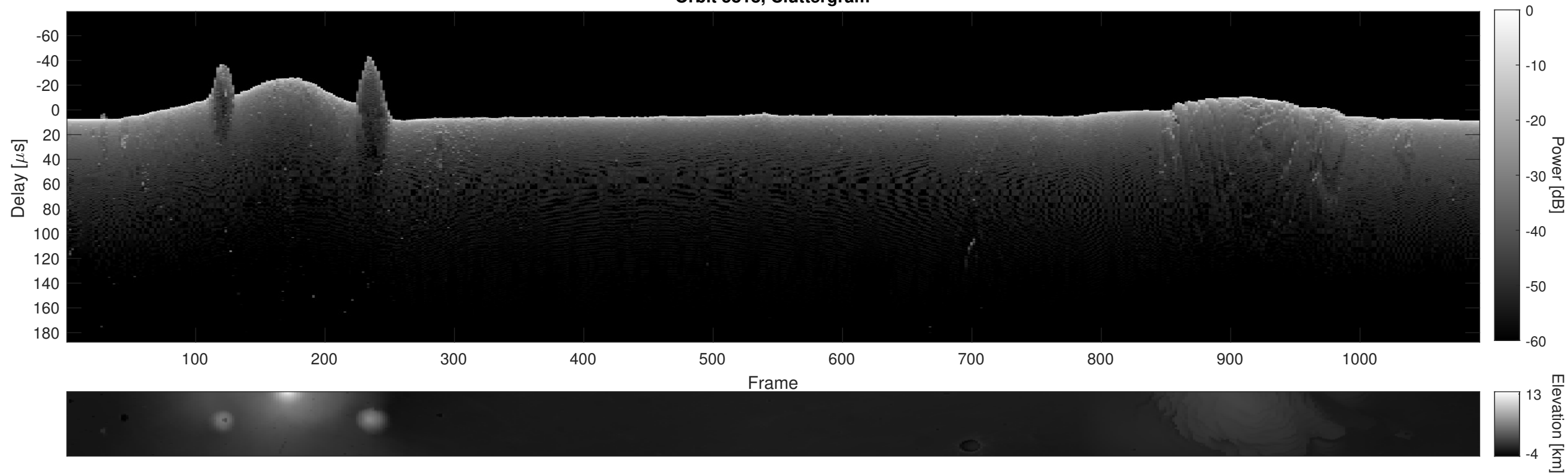
Orbit 5818, Cluttergram
