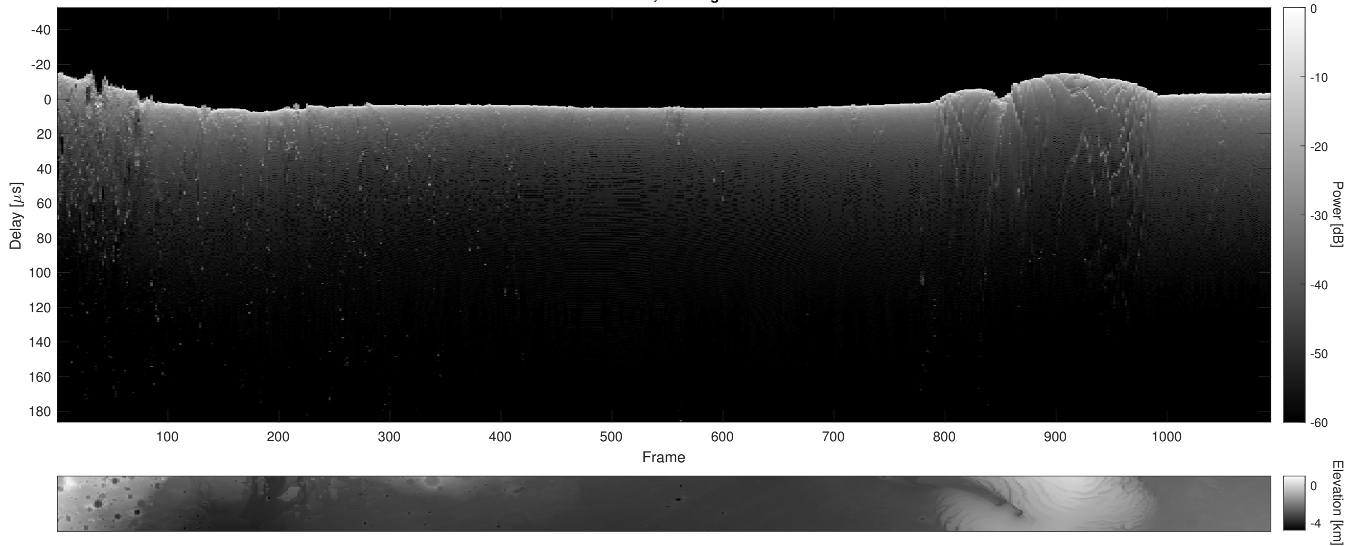
Orbit 5820, Cluttergram
