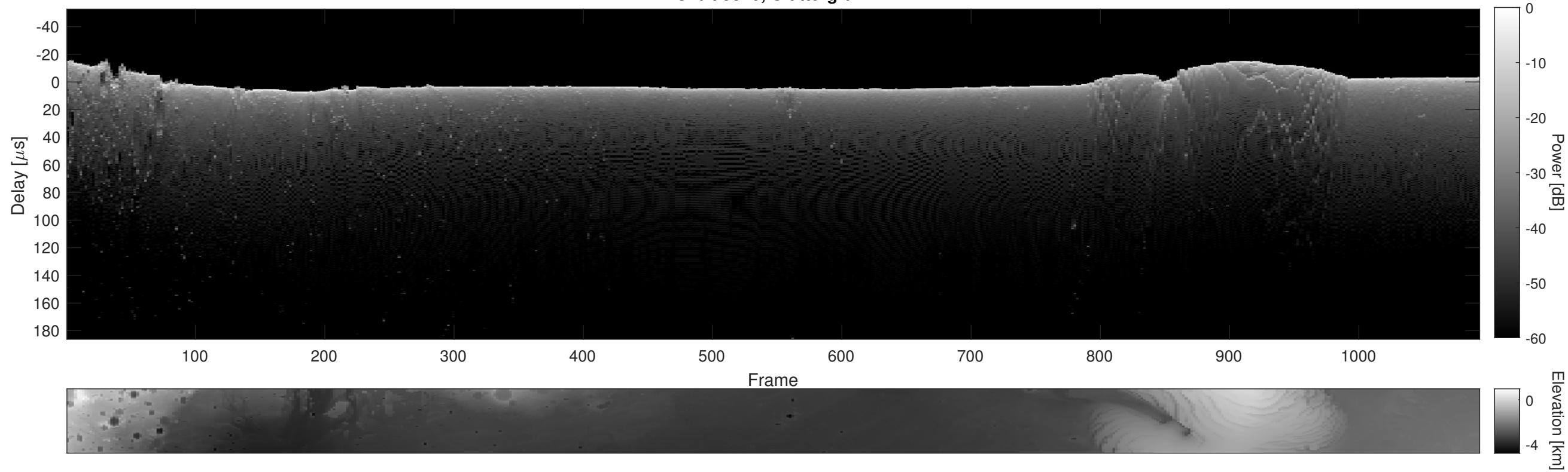
Orbit 5820, Cluttergram
