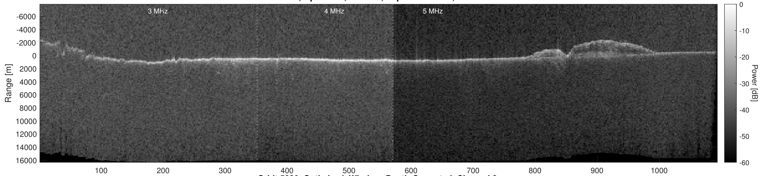
Orbit 5820, Optimized, Window, Depth-Corrected, Channel 2
