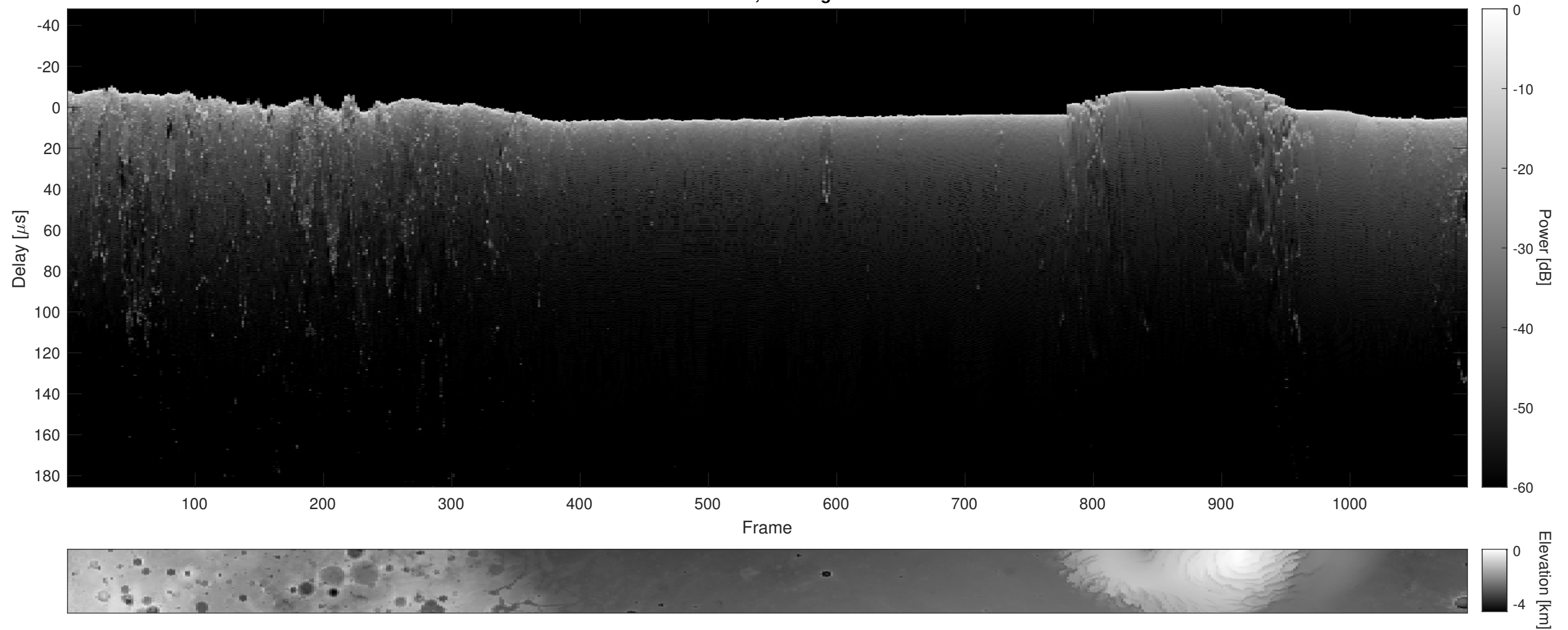
Orbit 5823, Cluttergram
