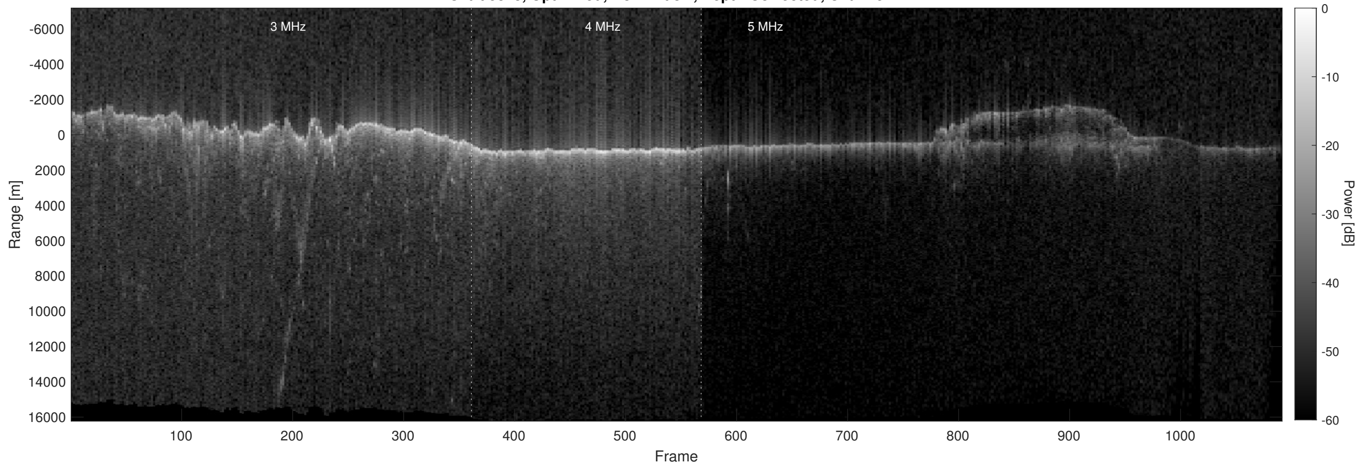
Orbit 5823, Optimized, No Window, Depth-Corrected, Channel 2
