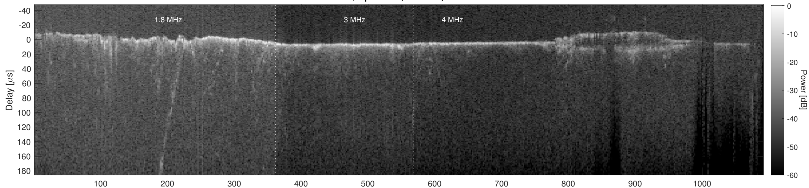
Orbit 5823, Cluttergram
