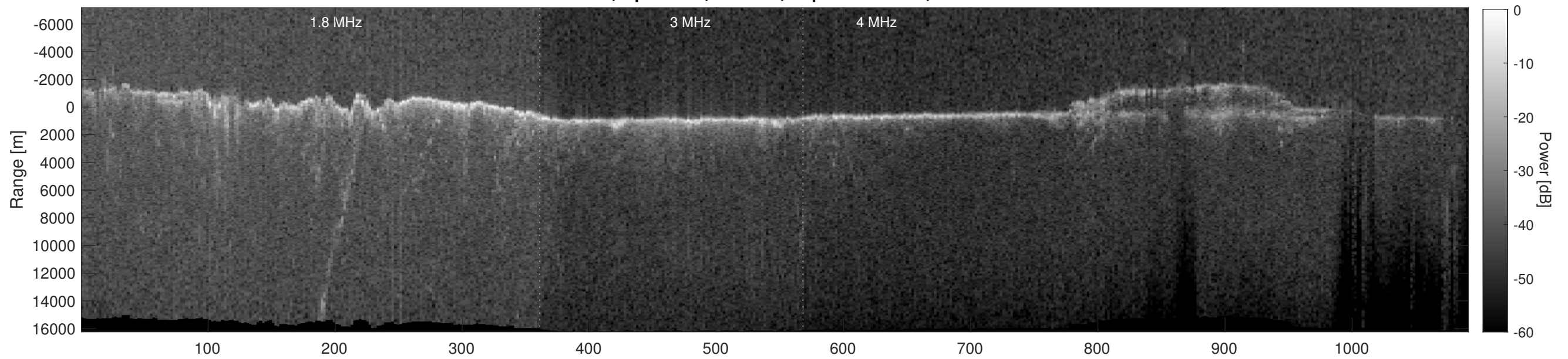
Orbit 5823, Depth-Corrected Cluttergram
