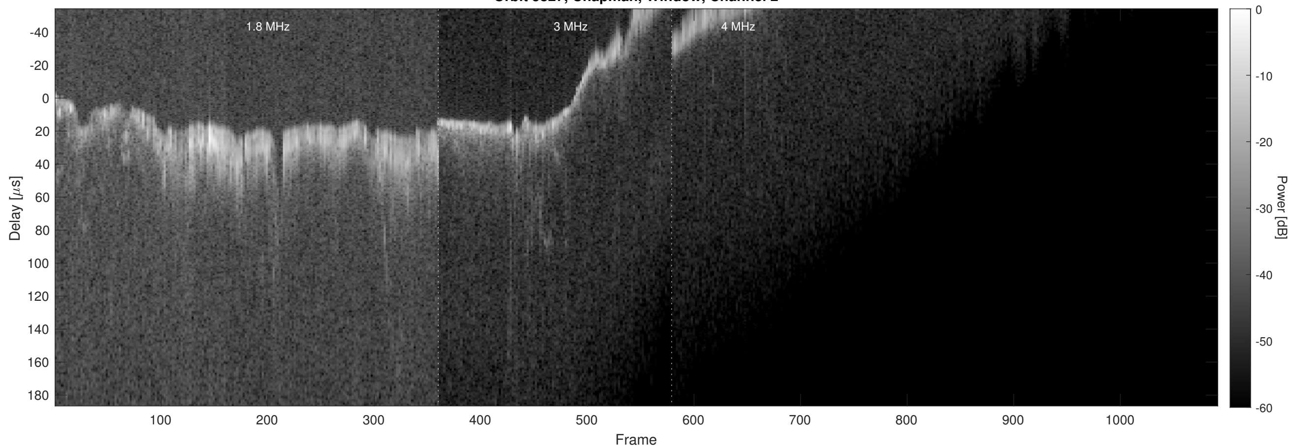
Orbit 5827, Chapman, Window, Channel 2
