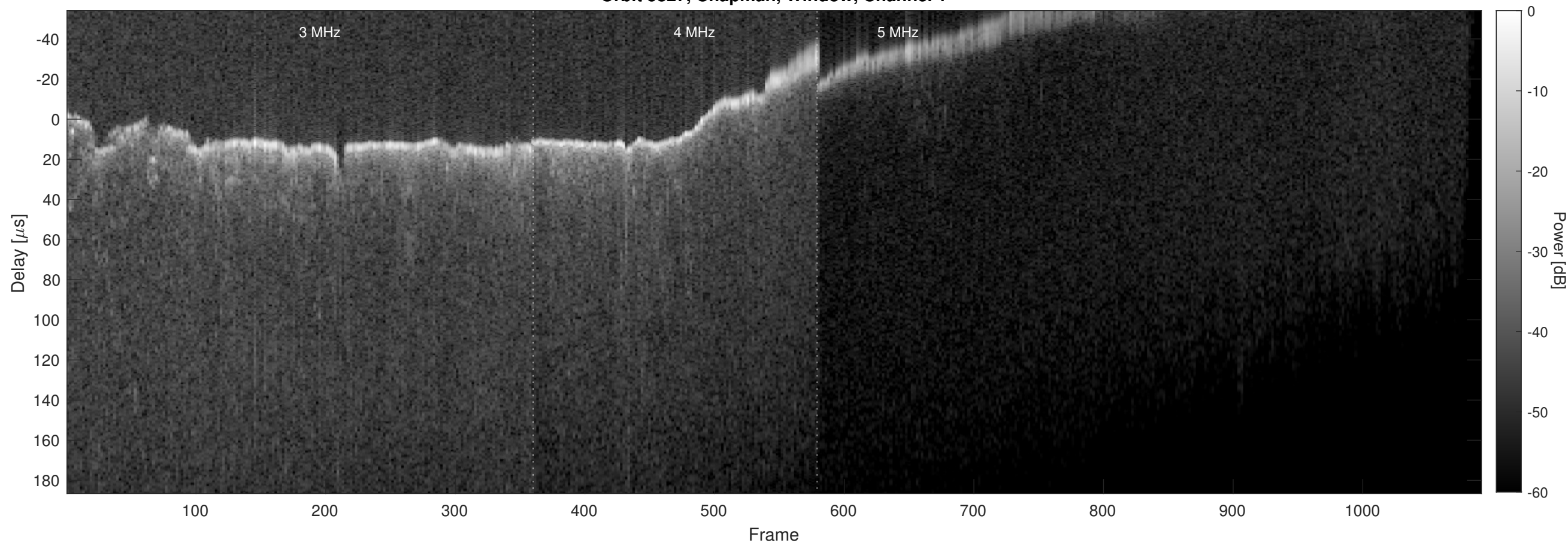
Orbit 5827, Chapman, Window, Channel 2
