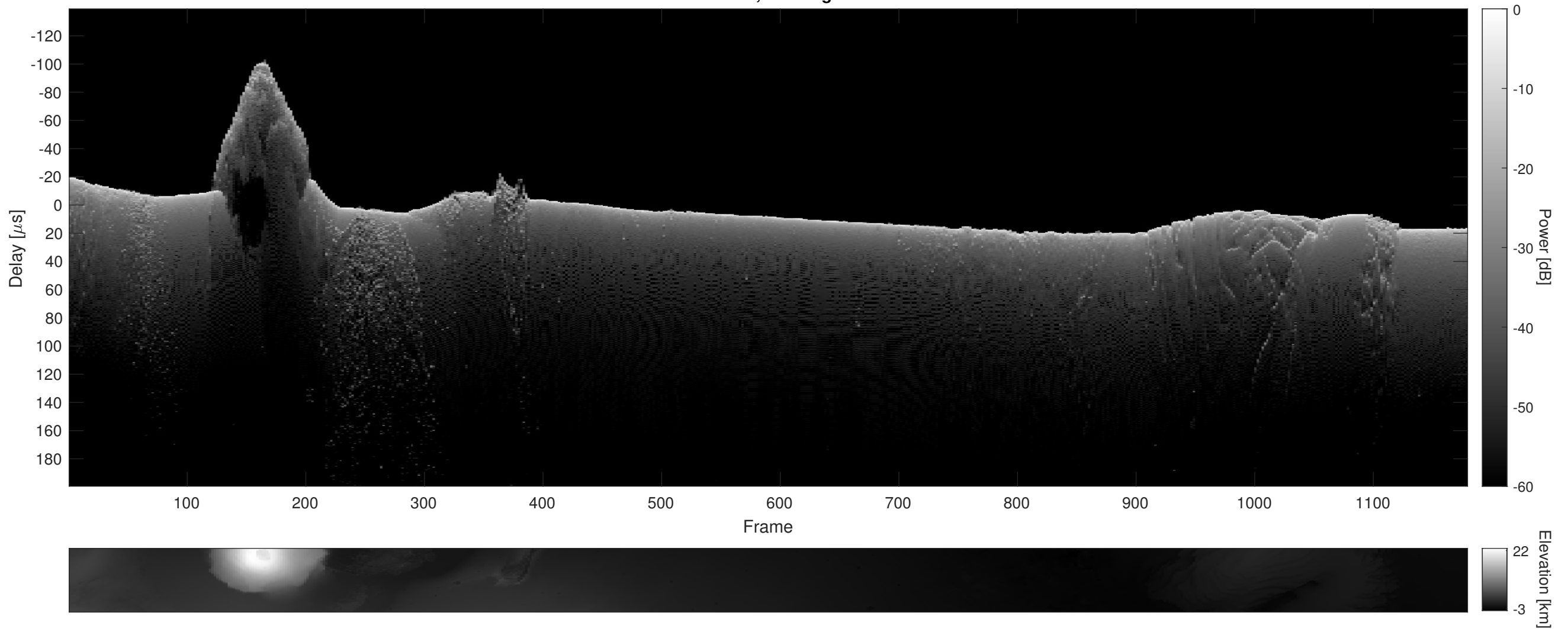
Orbit 5828, Cluttergram
